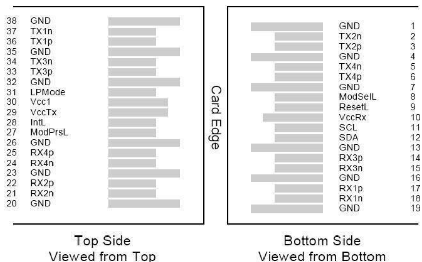
Figure 2: Pin Definitions.
